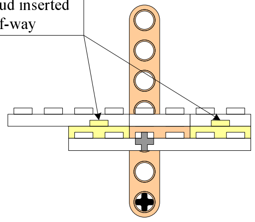
Cross-cut A-A
